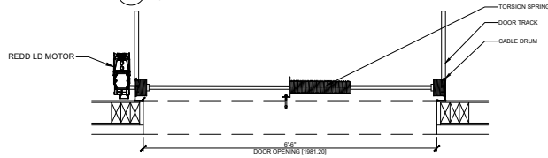
02 DOOR PLAN (ABOVE) SCALE: 1" = 1'
