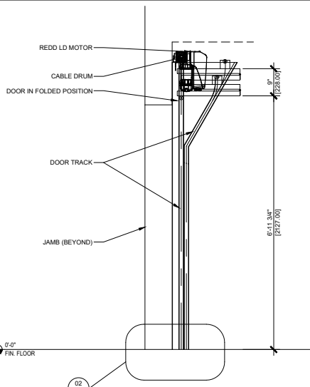
05 DOOR SECTION SCALE: 3/4" = 1'
