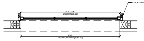
01 DOOR PLAN SCALE: 1" = 1'
