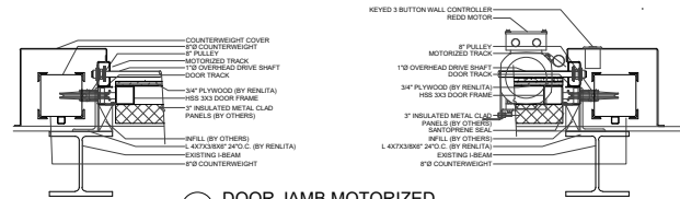
01 DOOR JAMB MOTORIZED SCALE: 1/2" = 1'
