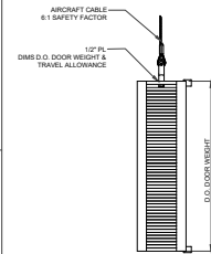
08 COUNTERWEIGHT TYP SCALE: 1-1/2" = 1'
