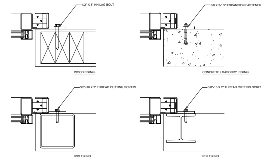
07 FIXING DETAILS TYP SCALE: 3" = 1'
