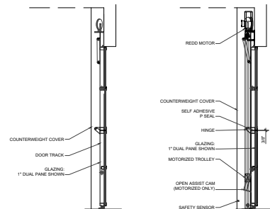
03 DOOR JAMB NON-MOTORIZED SCALE: 1-1/2" = 1'
