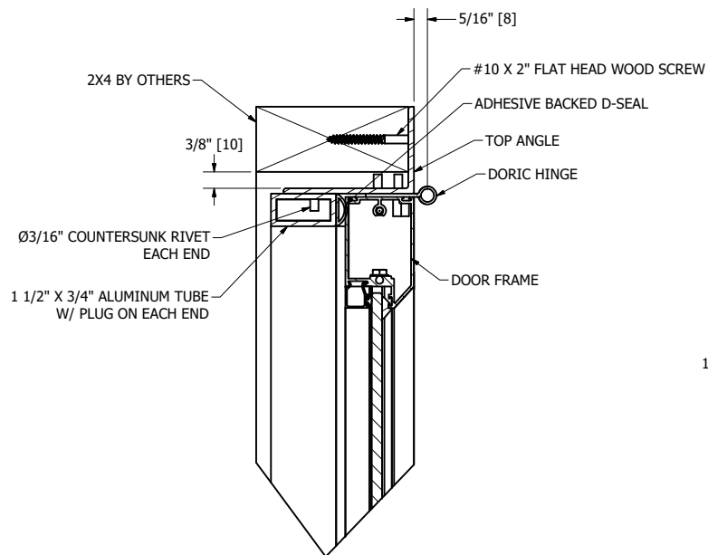
SECTION A-A SCALE 1/2
