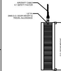
08 COUNTERWEIGHT TYP SCALE: 1/2" = 1'
