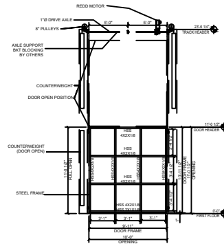
04 ELEVATION & SECTIONS MOTORIZED & NON SCALE: 1/4" = 1'
