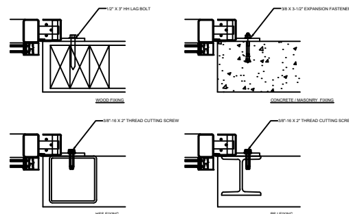
07 FIXING DETAILS TYP SCALE: 3/4" = 1'
