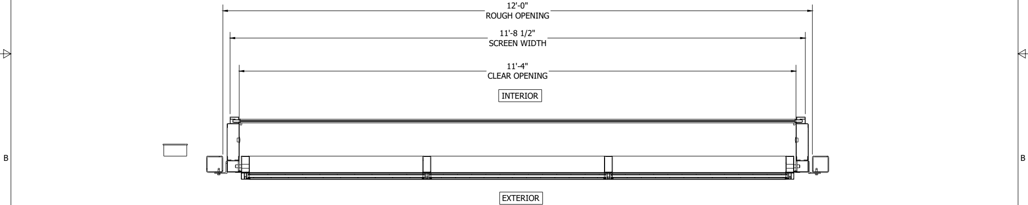
02 PLAN VIEW BELOW ACTUATOR
