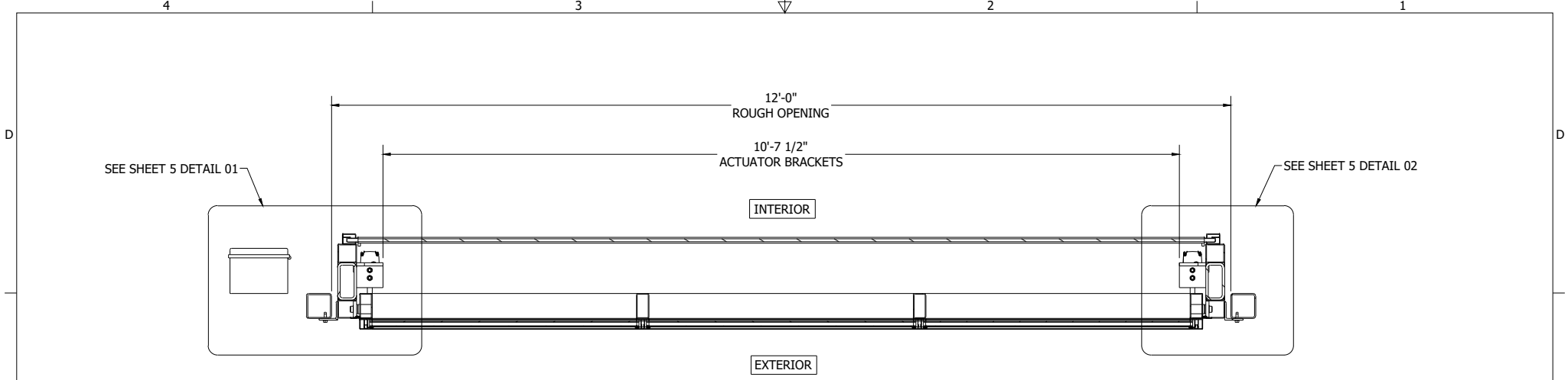
01 PLAN VIEW ABOVE ACTUATOR
