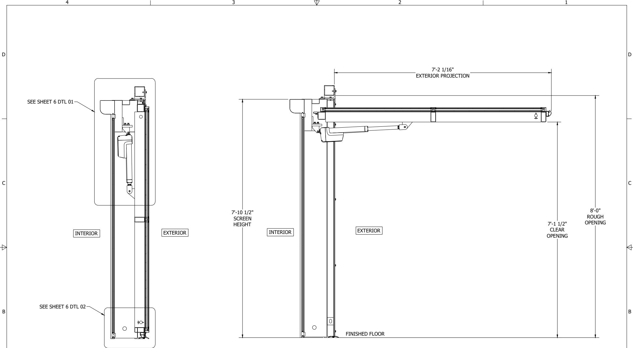
01 SECTION VIEW CLOSED
