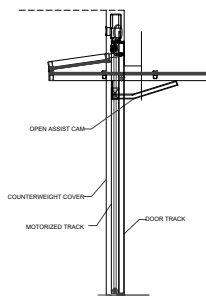
04 ELEVATION & SECTIONS MOTORIZED & NON SCALE: 1/2\"/>
