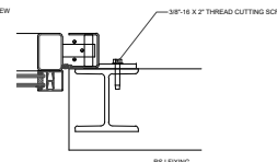
07 FIXING DETAILS TYP SCALE: 2\"/>
