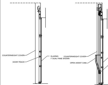
03 DOOR JAMB NON-MOTORIZED SCALE: 1-1/2\"/>
