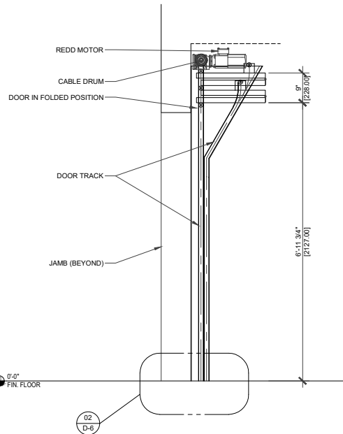
05 DOOR SECTION SCALE: 3/4" = 1'
